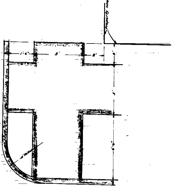
PLAN SIDEWALK AND CURB RETURN AT B SCALE 3/8" = 1'
