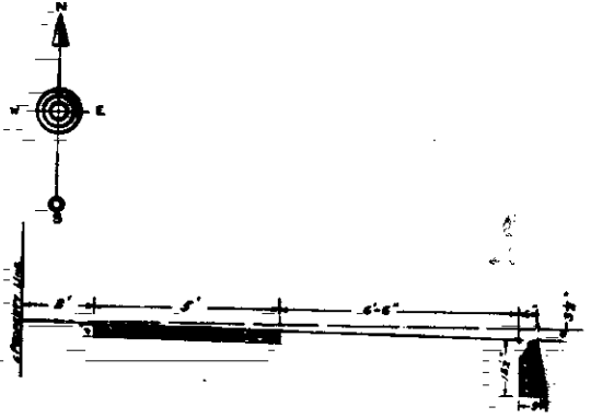
ENLARGED SECTION OF SIDEWALK AND CURB AT A.A. SCALE 3/8" = 1'
